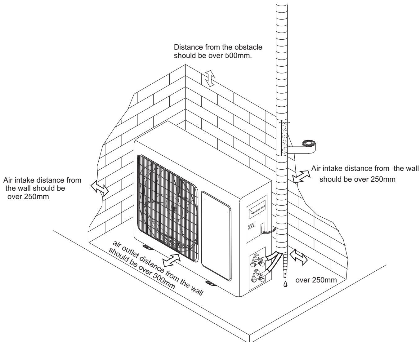
outdoor unit
