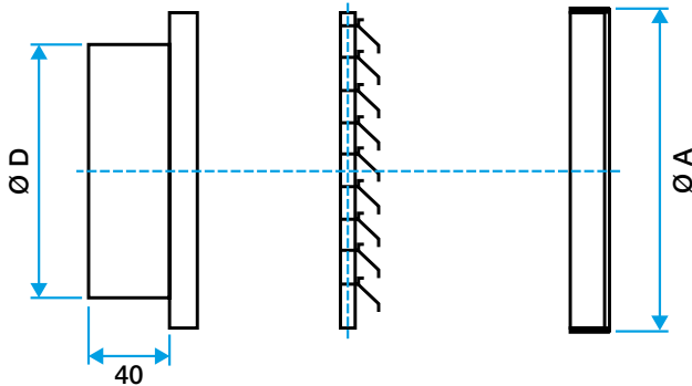
AR 637 grille diameter 125 to 315 mm
