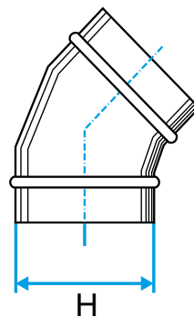
Dimensional drawing oblong horizontal 45° bend
