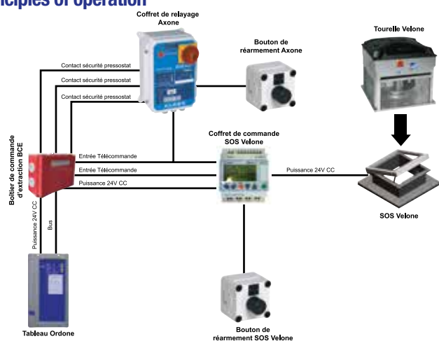
Schematic diagram of AXONE and SOS VELONE reset units
