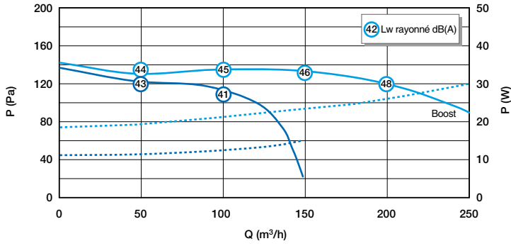
Aerodynamic and acoustic curve EasyHOME Auto Classic
