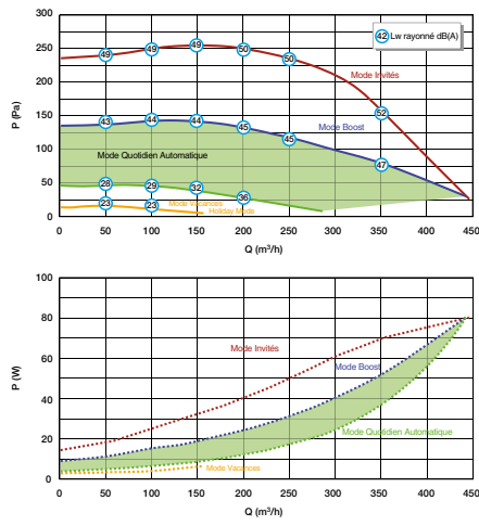
Aerologic and acoustic curve EasyHOME PureAIR COMPACT Connect
