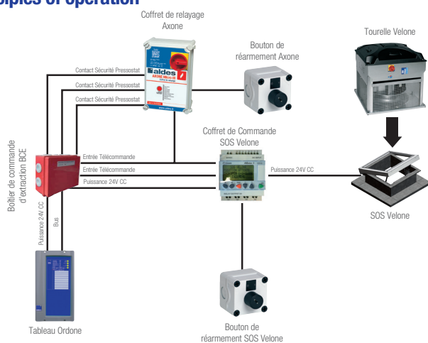
Schematic diagram of AXONE and SOS VELONE reset units
