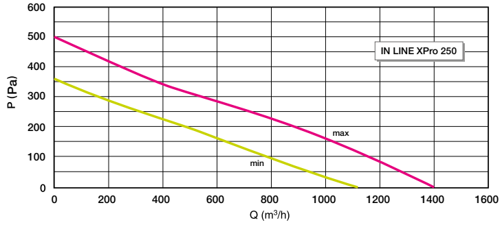
Aeraulic curve XPro 250
