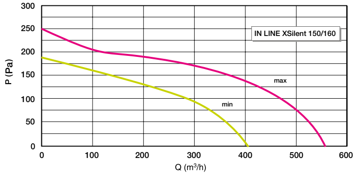
Aeraulic curve XSilent 150
