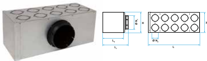
Distribution unit OPTIFLEX 20 connections
