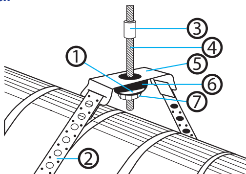
Installation drawing for perforated strip
