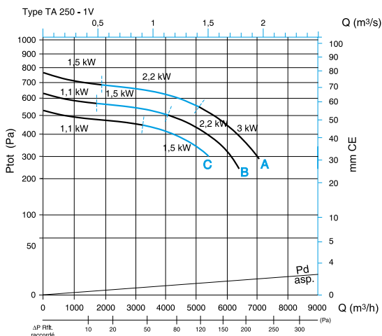
Aeraulic properties ProtectONE® TA 250 - 1SP
