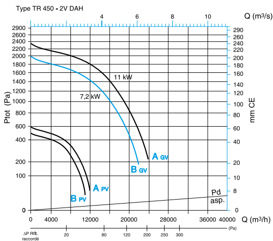
Aeraulic properties ProtectONE® TR 450 - 2SP - DAH
