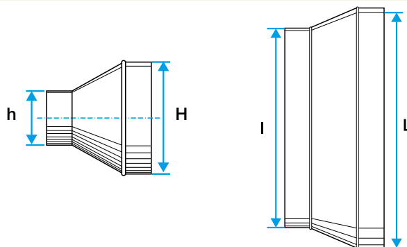
Dimensional diagram Oblong Concentric Reducer
