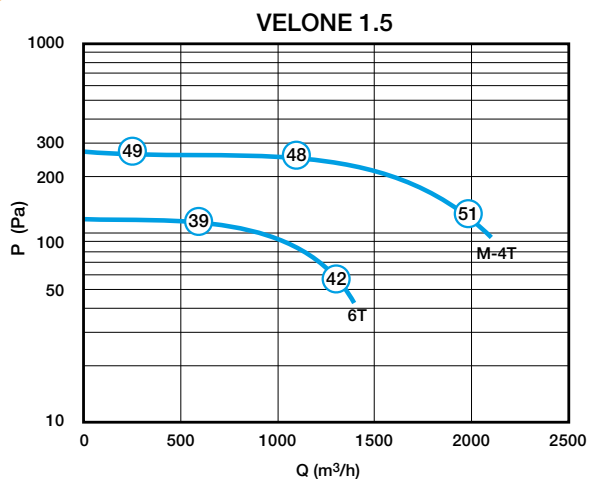
Aeratic and acoustic properties VELONE 1.5M 0.24 KW+IP
