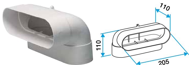
Coude vertical 90°
