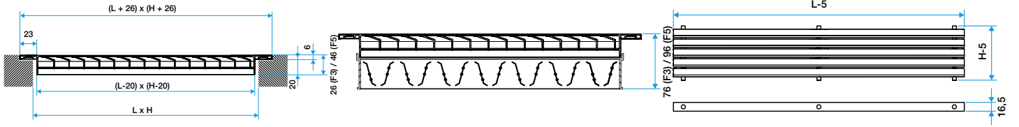
Gridlined Exhaust
