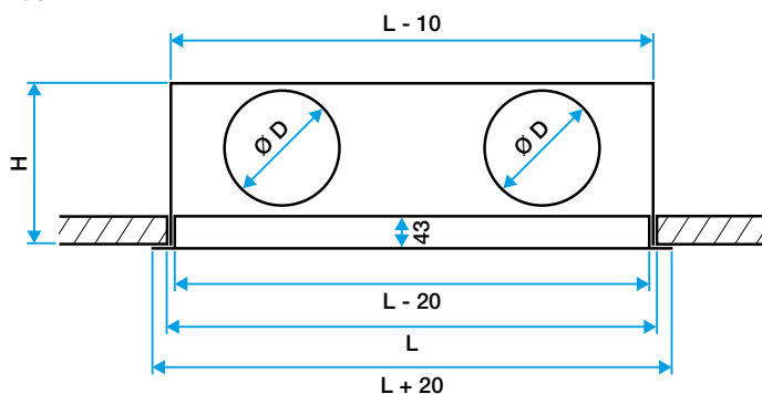
Plénum LINED
