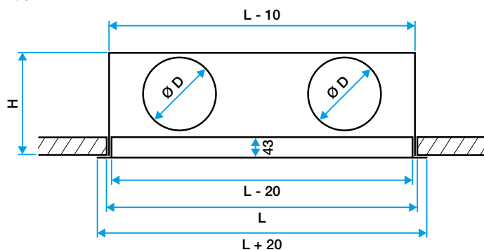
Plenum LINED
