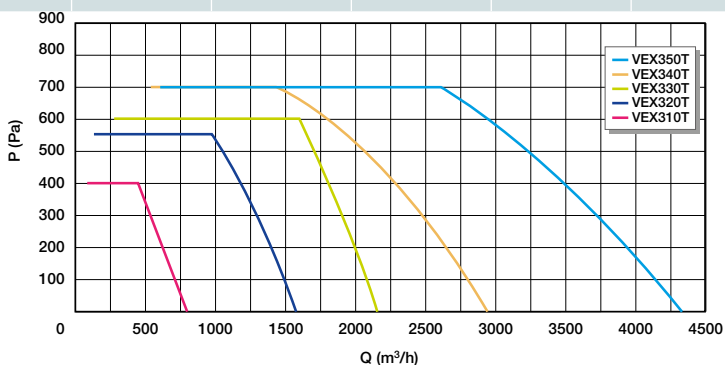
Aeraulic characteristics VEX300T
