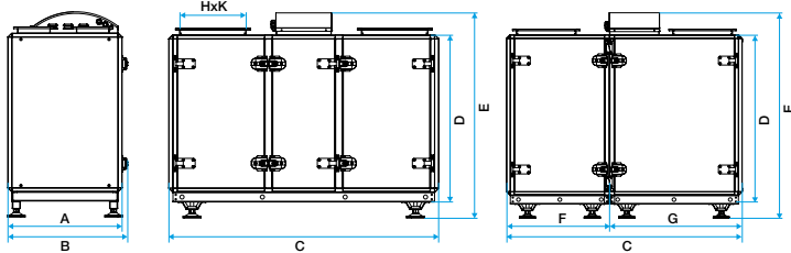
Dimensions VEX700T
