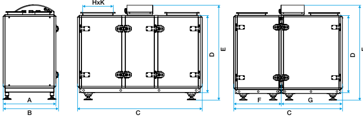
Dimensions VEX700T
